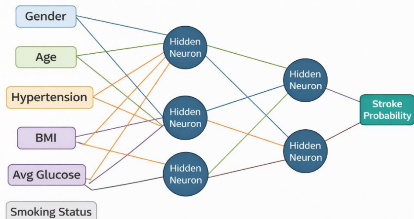
Neural Network for Stroke Prediction
